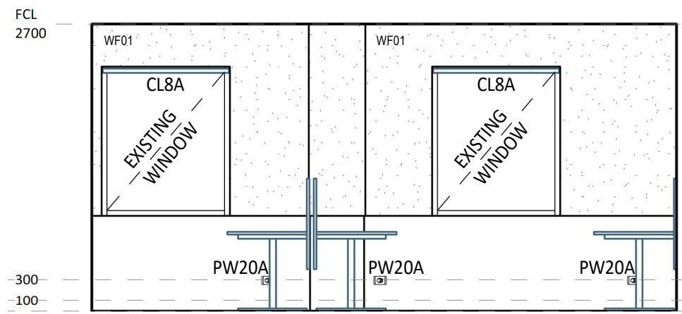
7 ELEVATION DETAIL 60-03 1 : 50
