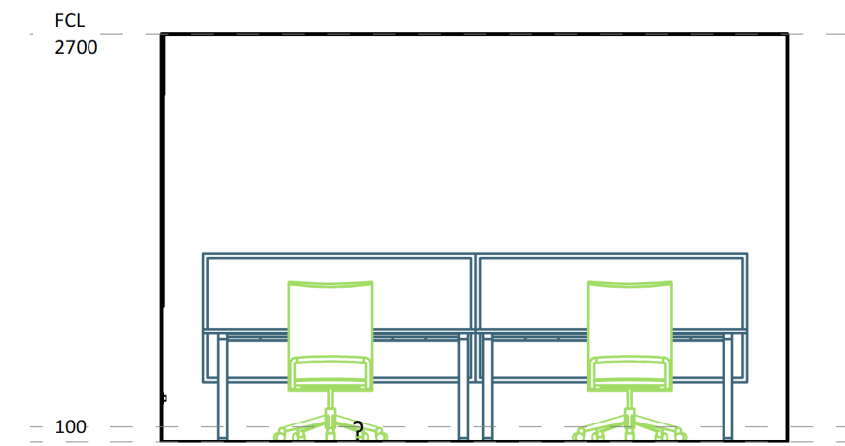
8 ELEVATION DETAIL 60-03 1 : 50
