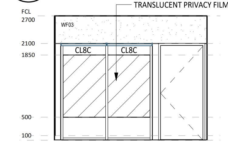
5 ELEVATION DETAIL 1 : 50
