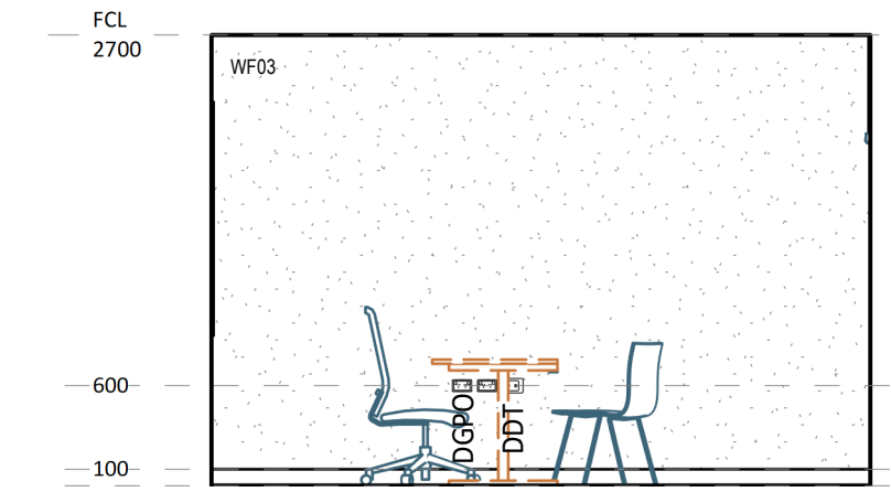
4 ELEVATION DETAIL 1 : 50
