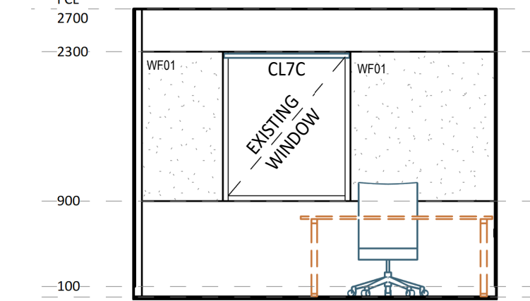
3 ELEVATION DETAIL 1 : 50
